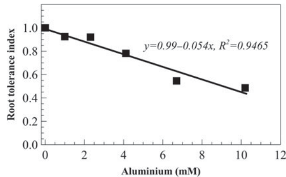
Figure 3. Root tolerance index of rambutan at different aluminium concentrations.
